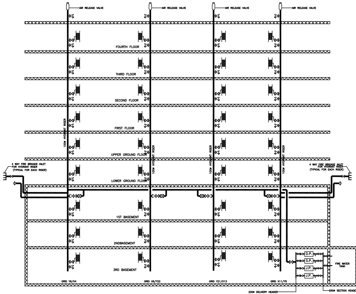
SCHEMATIC OF HYDRANT SYSTEM
