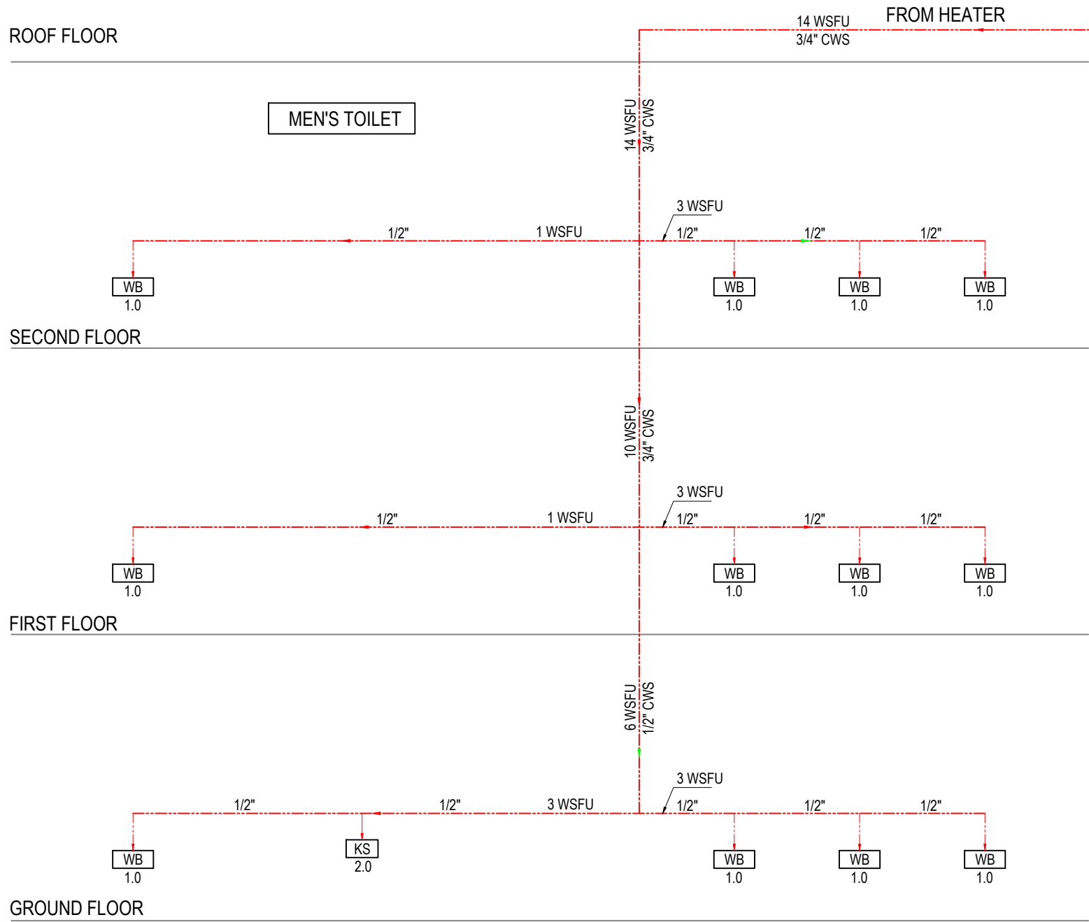
SCHMATIC RISER DIAGRAM HOT WATER SUPPLY (HWS) SYSTEM
