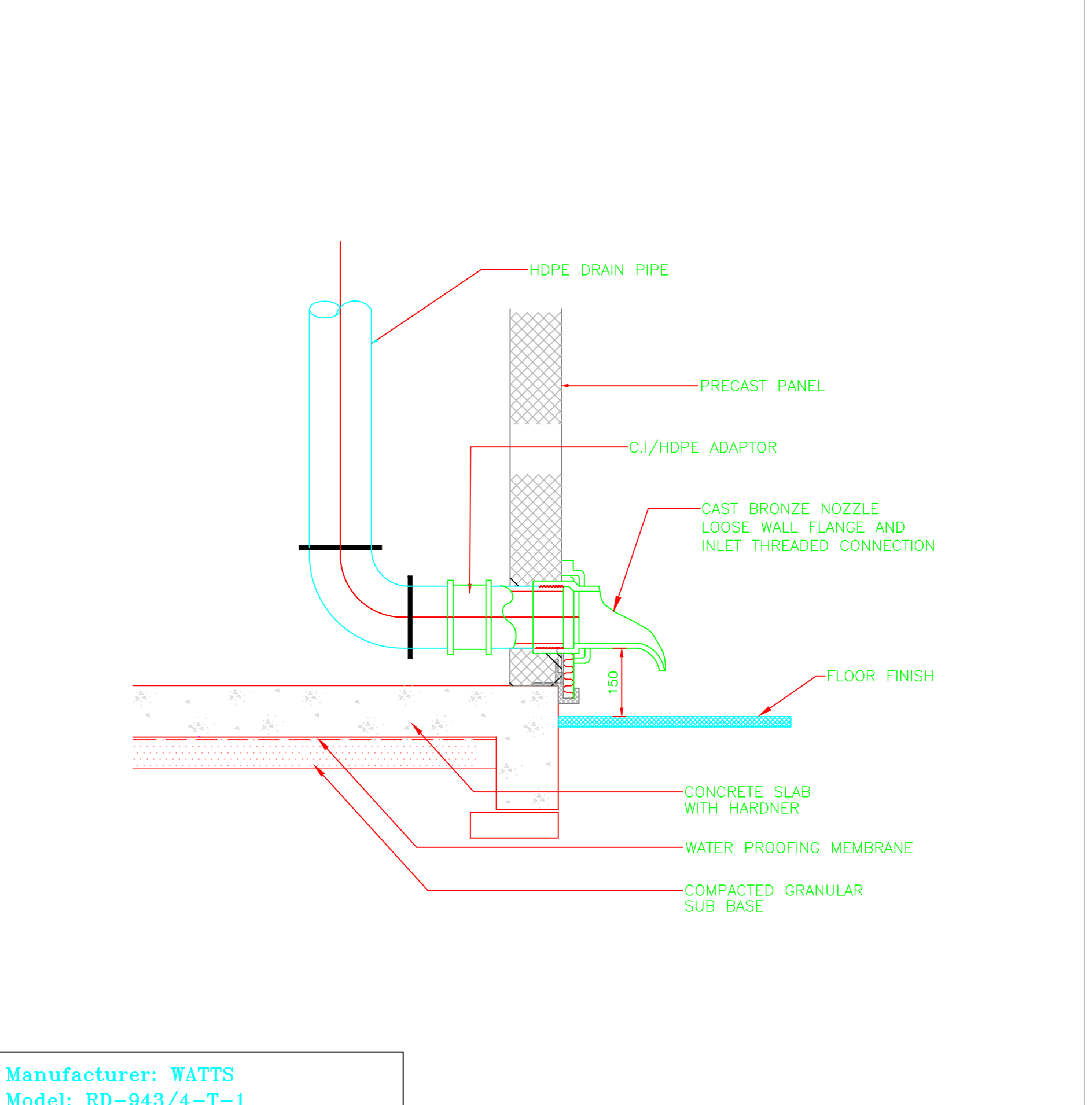
P9 - RAIN WATER SHOE
