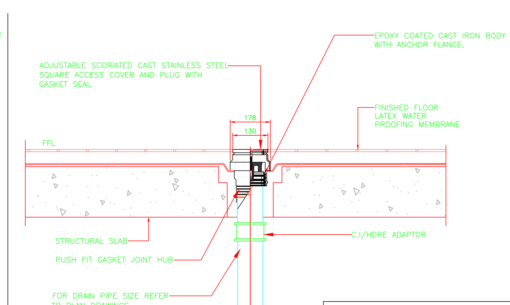
P4 - FLOOR CLEANOUT
