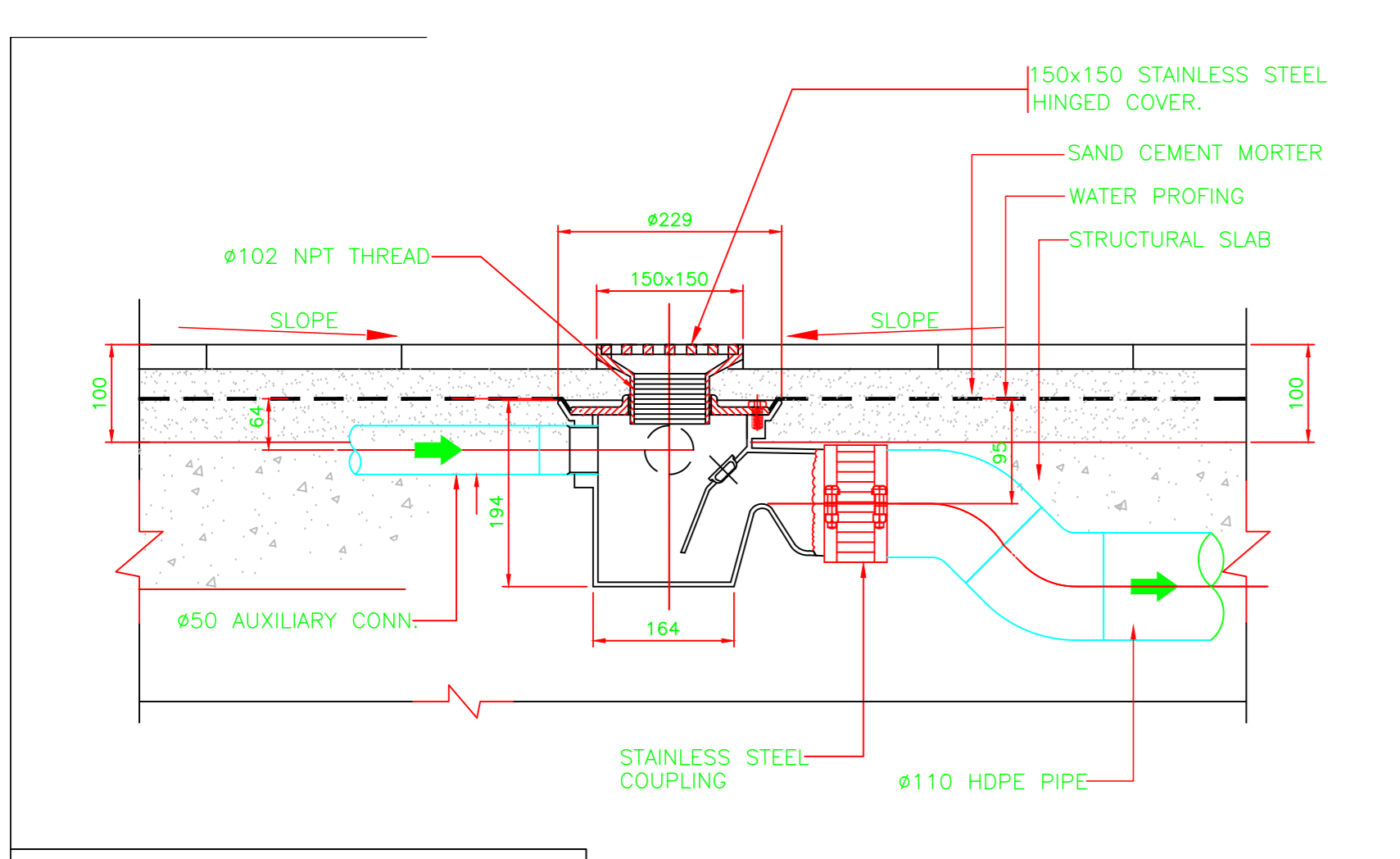
P1-FLOOR DRAIN (BUILT IN TRAP - AUXILIARY INLETS)
