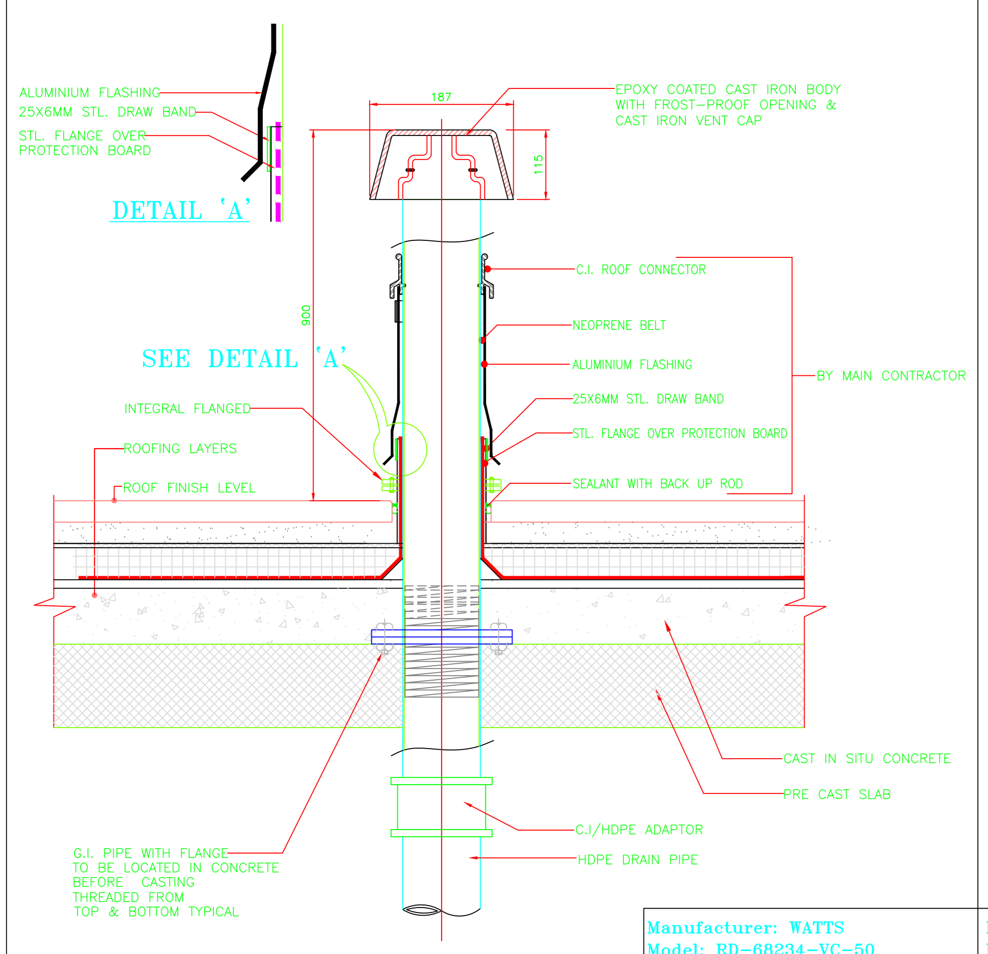
P6 - ROOF VENT TERMINAL
