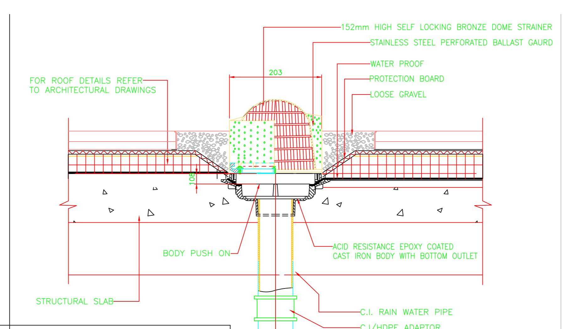
P5 - 03", 04" ROOF DRAIN
