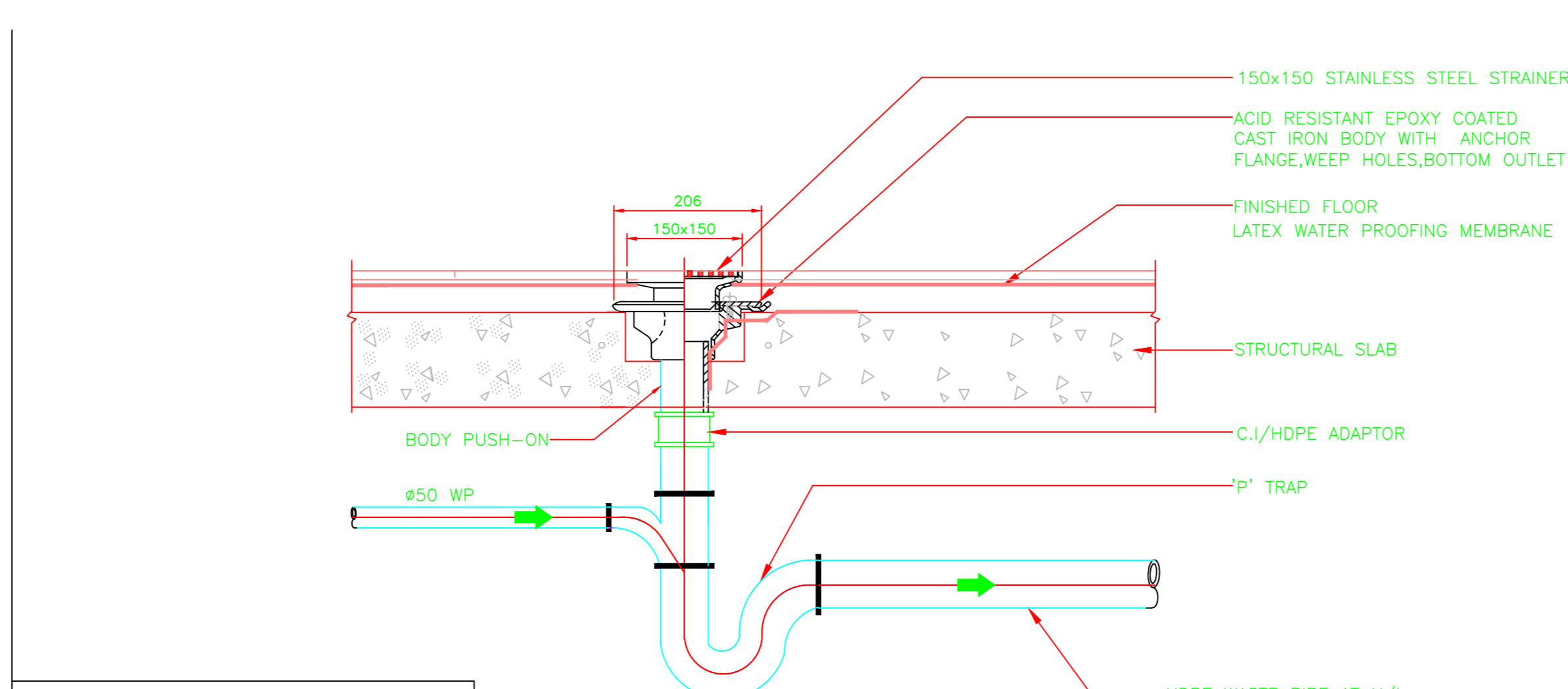
P2-FLOOR DRAIN (TRAP AT H/L)
