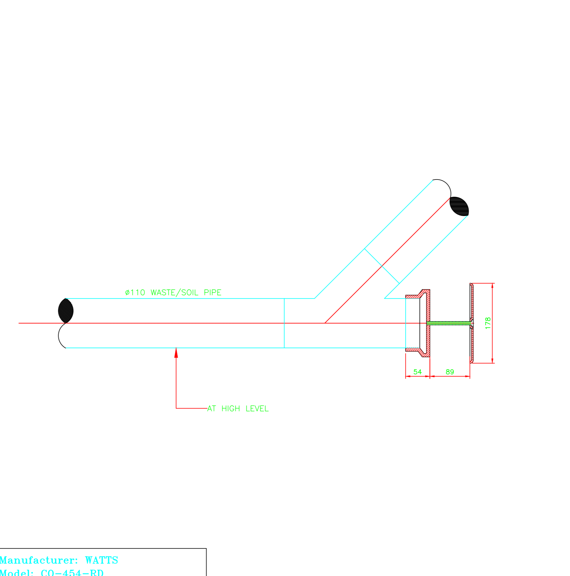
P7 - RODDING EYE (H/L CLEAN-OUT)
