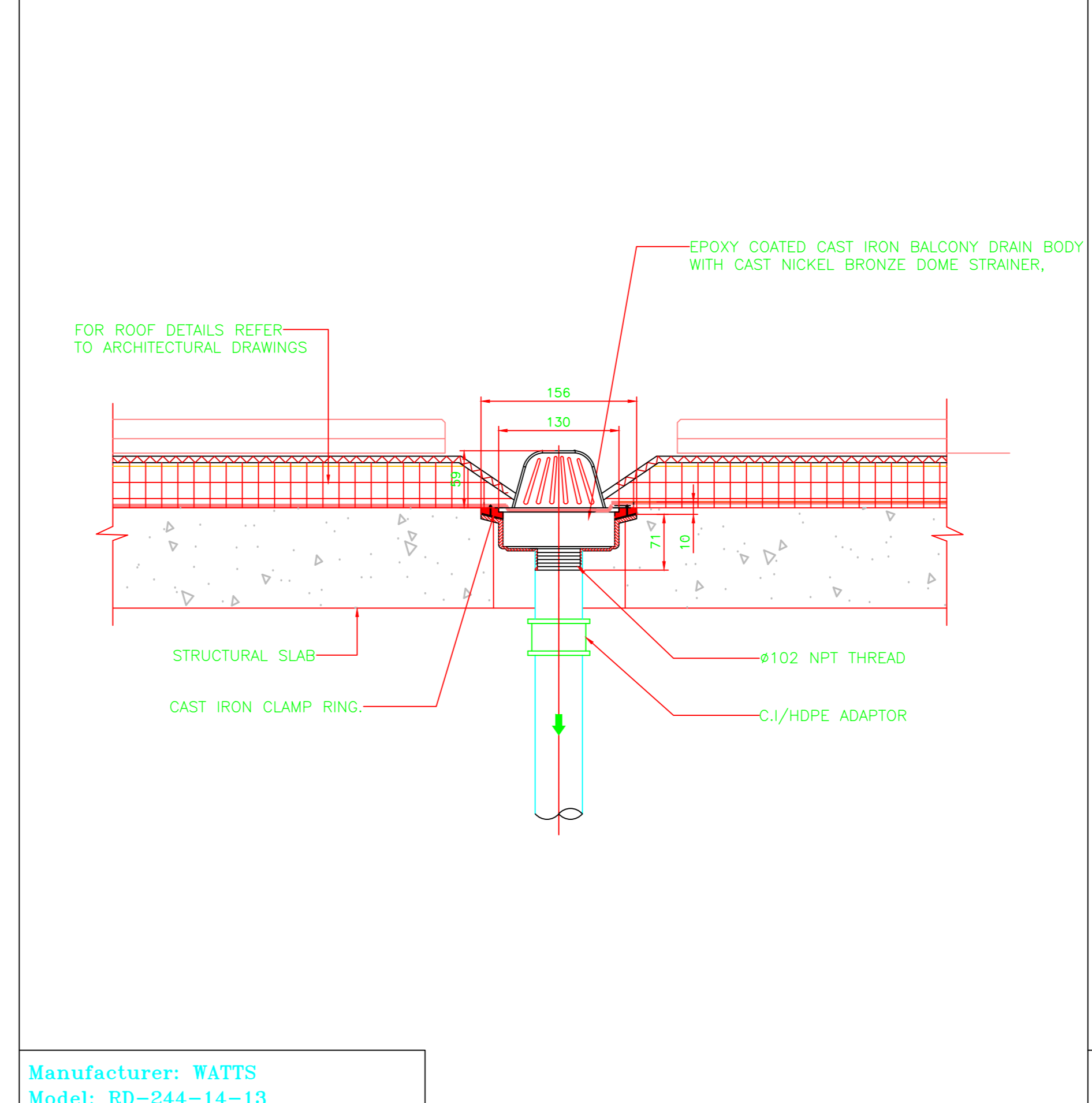
P8 - BALCONY DRAIN
