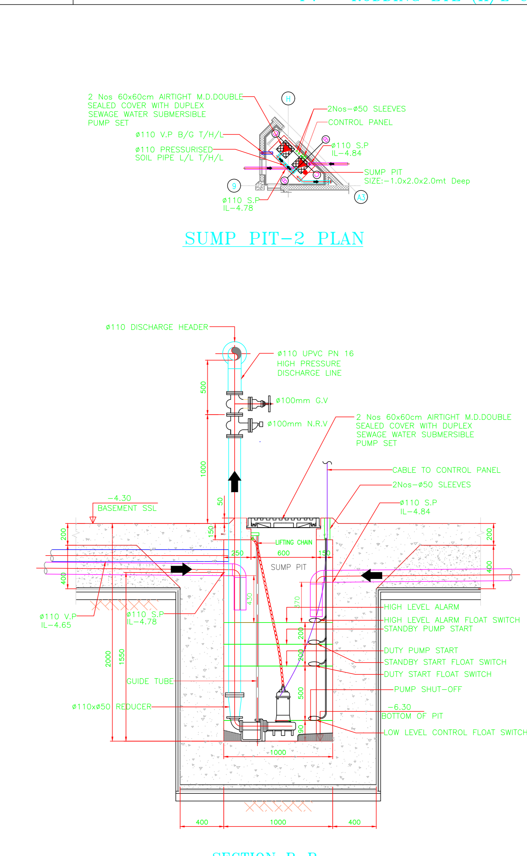
SECTION B-B
