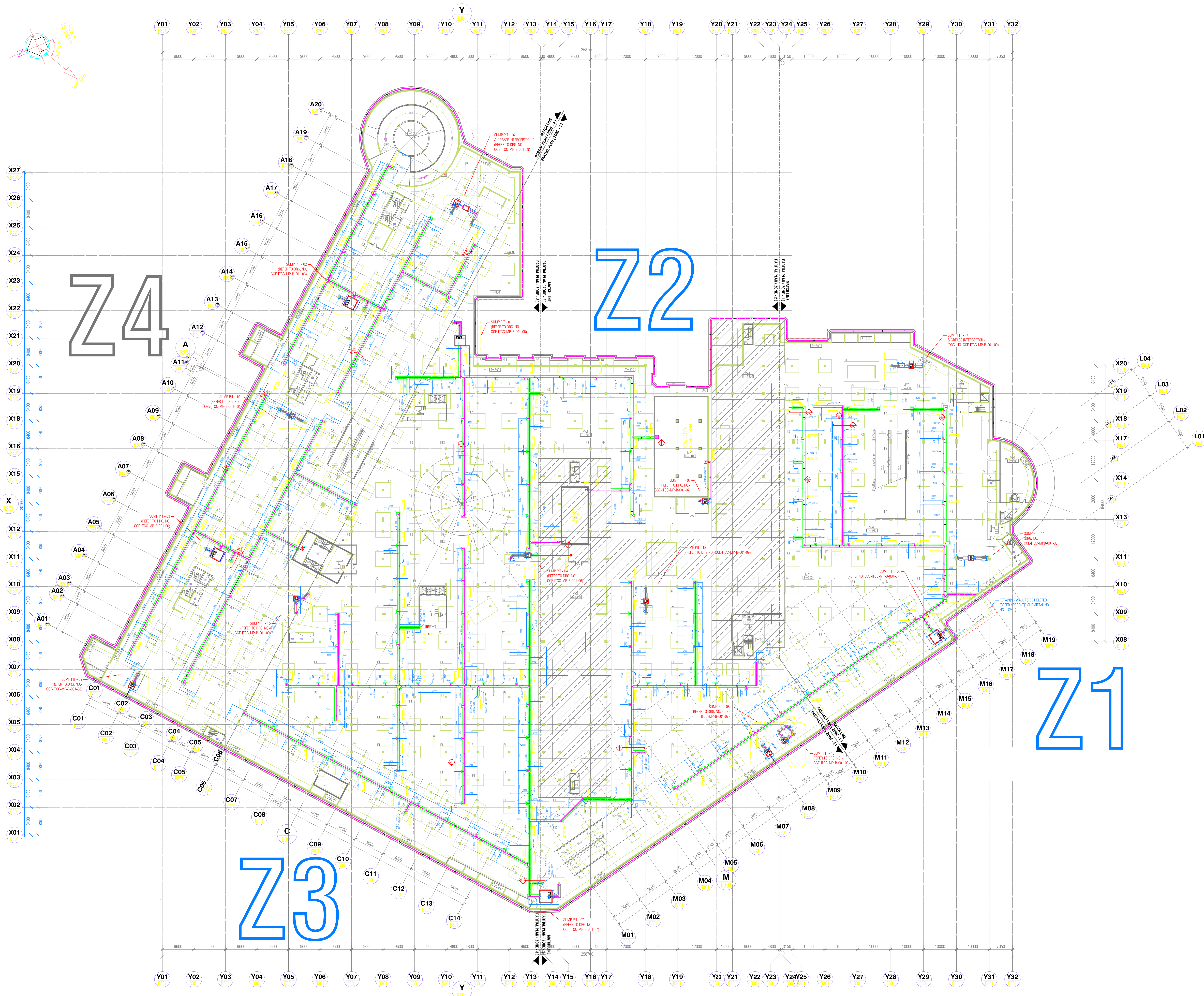
TRENCH, SUMP PIT & GREASE INTERCEPTOR GENERAL LAYOUT 3RD BASEMENT DRAINAGE SYSTEM SCALE=1:400
