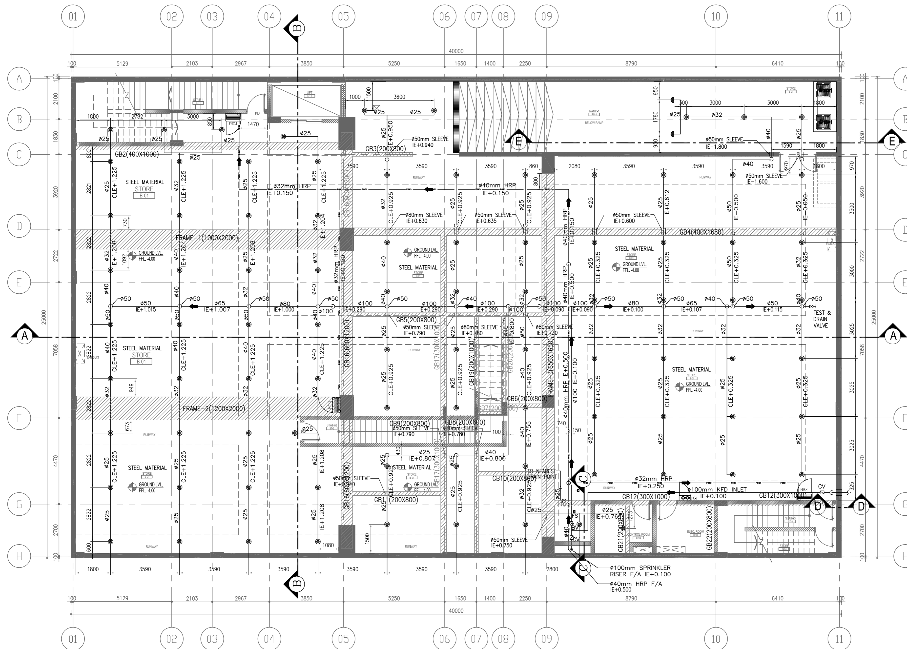
BASEMENT FLOOR PLAN FIRE PROTECTION LAYOUT SCALE: 1:100
