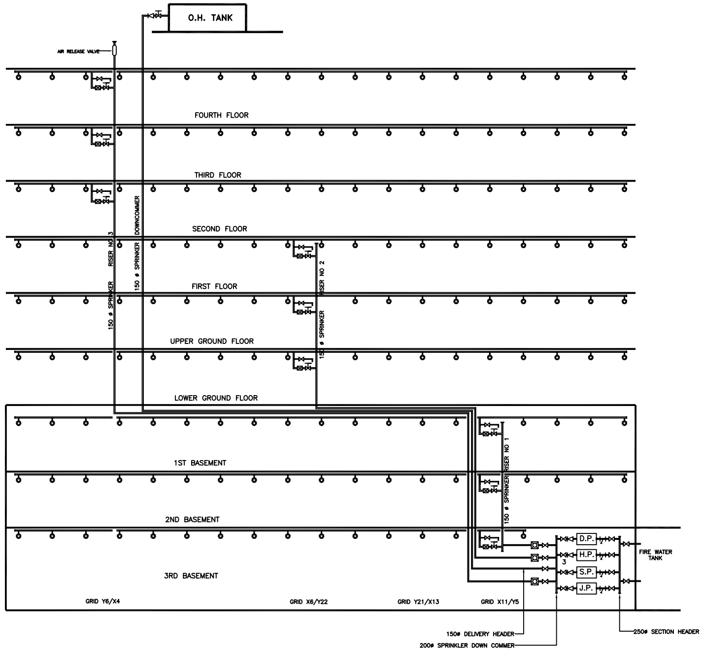
SCHEMATIC OF SPRINKLER SYSTEM
