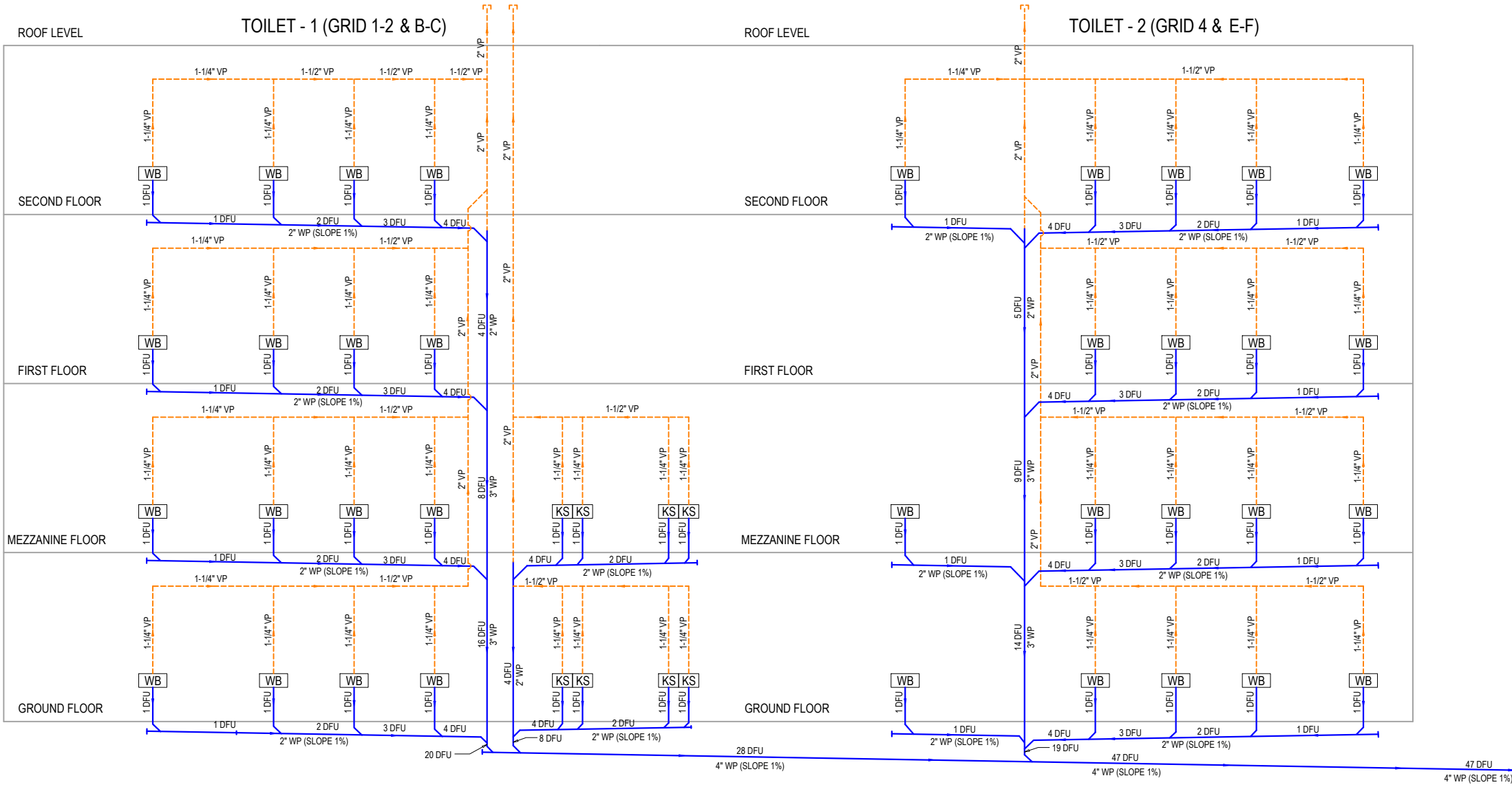
GREY WATER SCHEMATIC DIAGRAM
