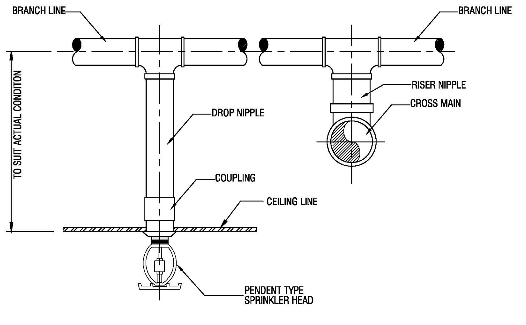
9 PENDENT TYPE SPRINKLER DETAIL G-PP002 N.T.S.
