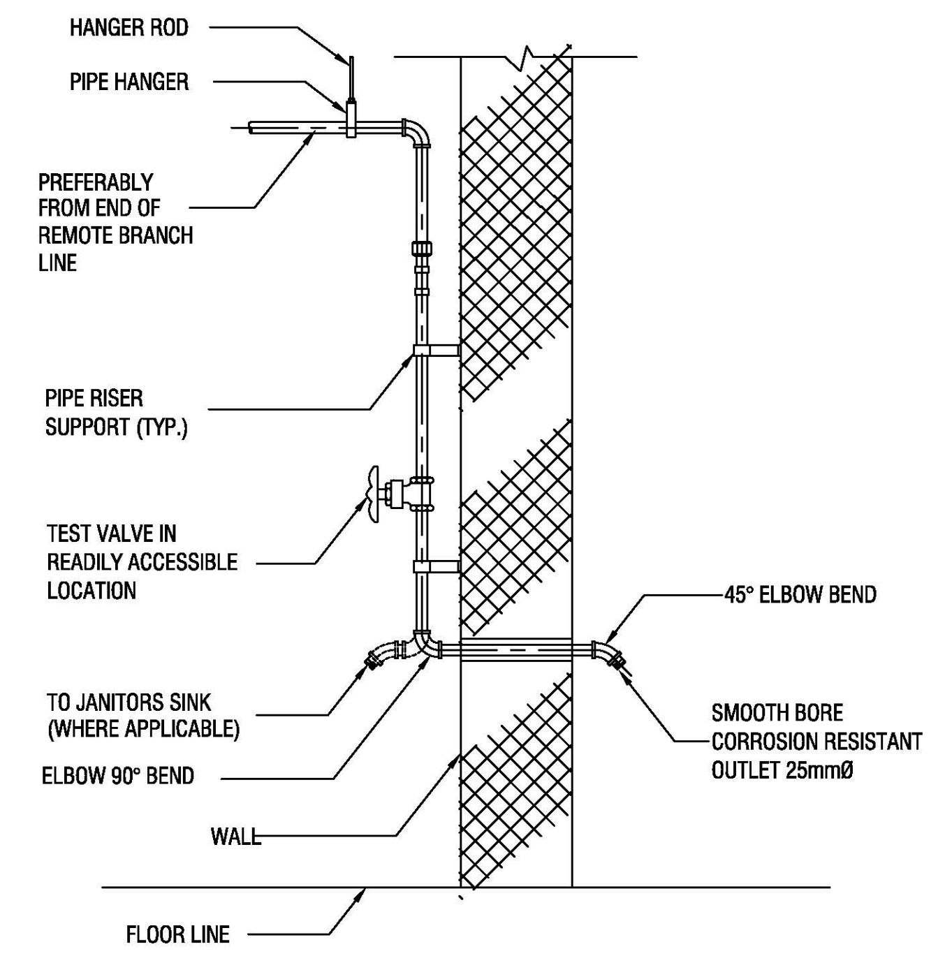
8 INSPECTOR'S TEST PIPE G-PP002 N.T.S.
