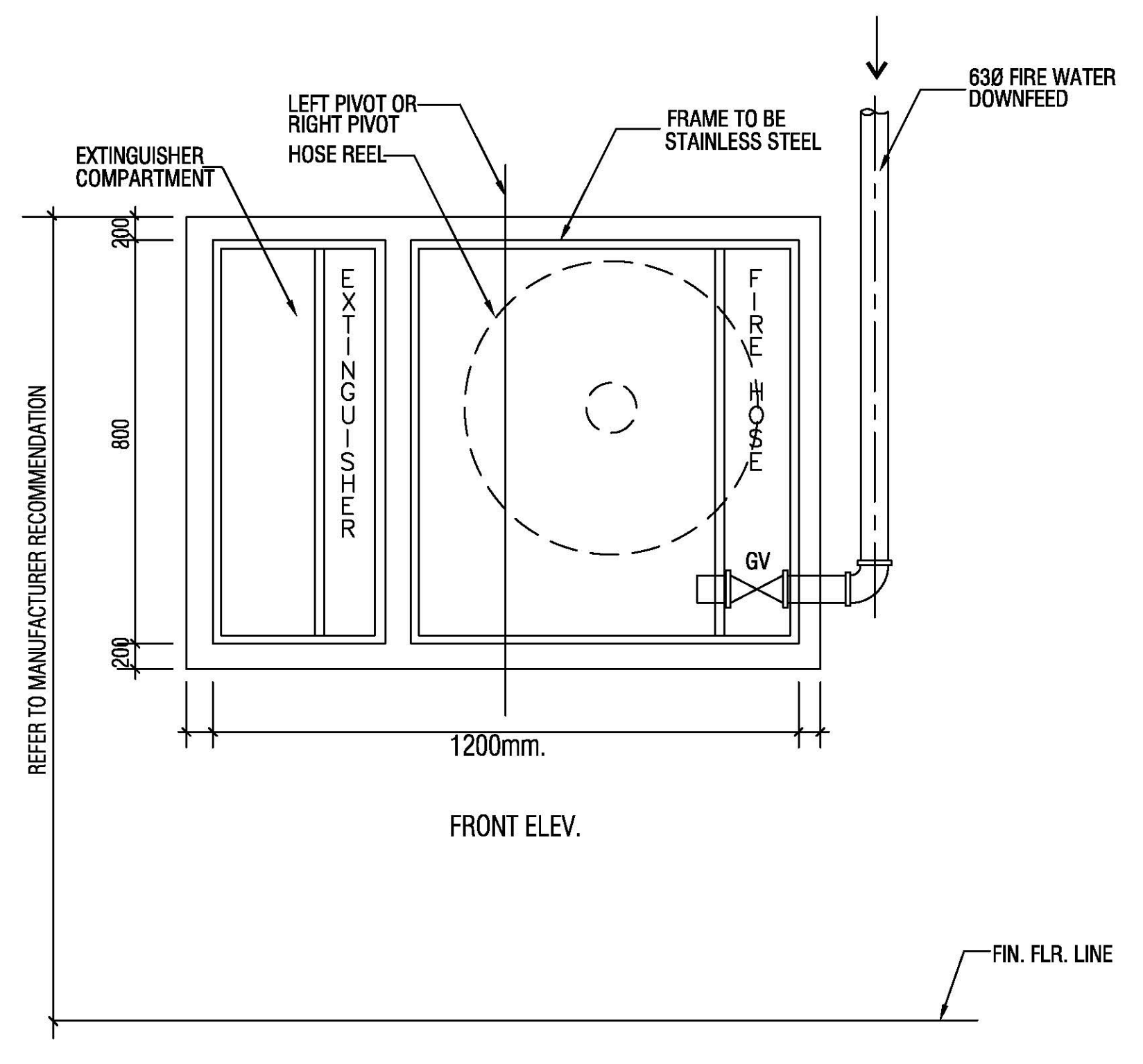
5 FIRE HOSE REEL DETAIL G-PP002 N.T.S.
