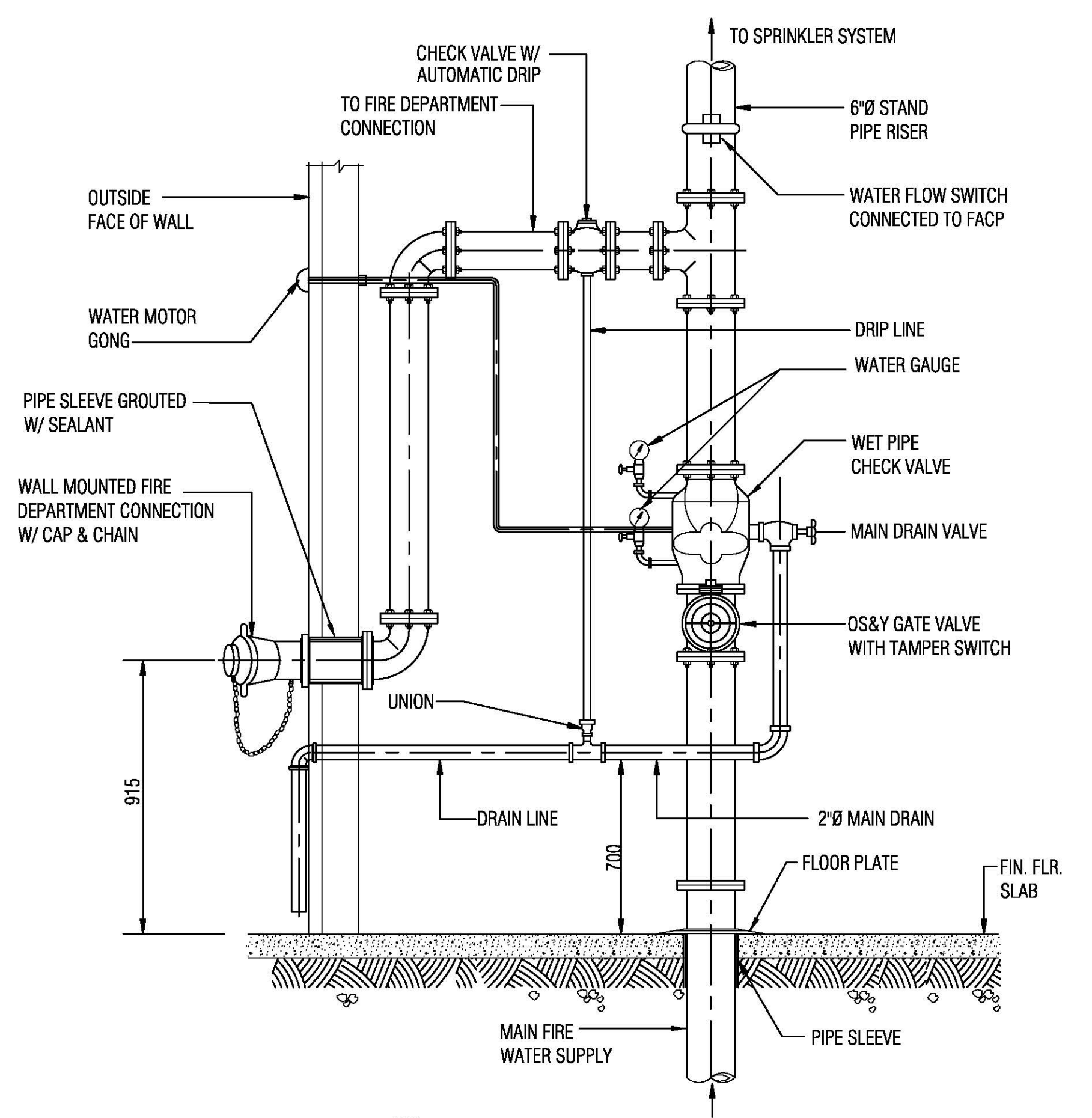
4 FIRE ALARM CHECK VALVE DETAIL G-PP002 N.T.S.
