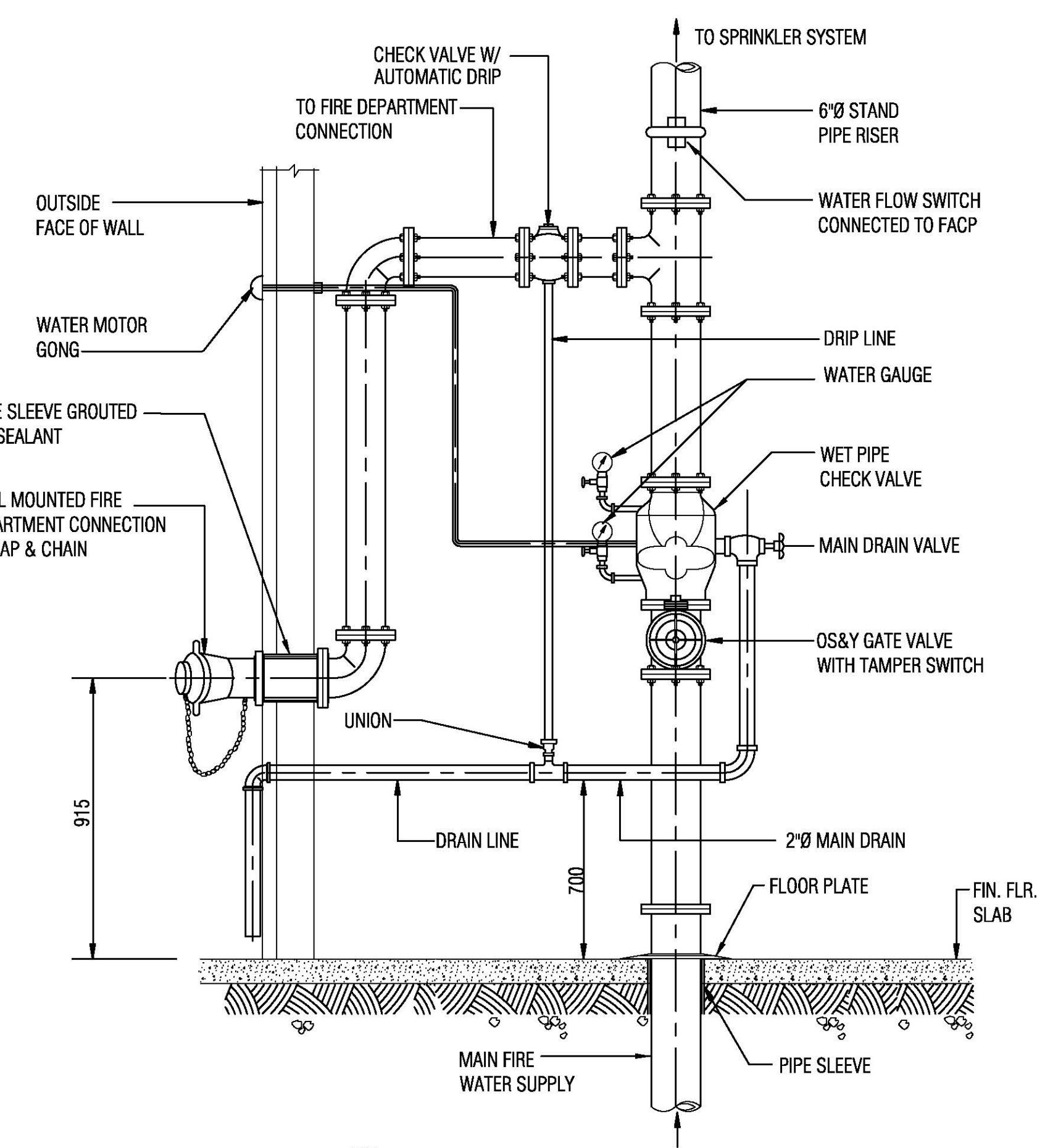
4 FIRE ALARM CHECK VALVE DETAIL G-PP002 N.T.S.
