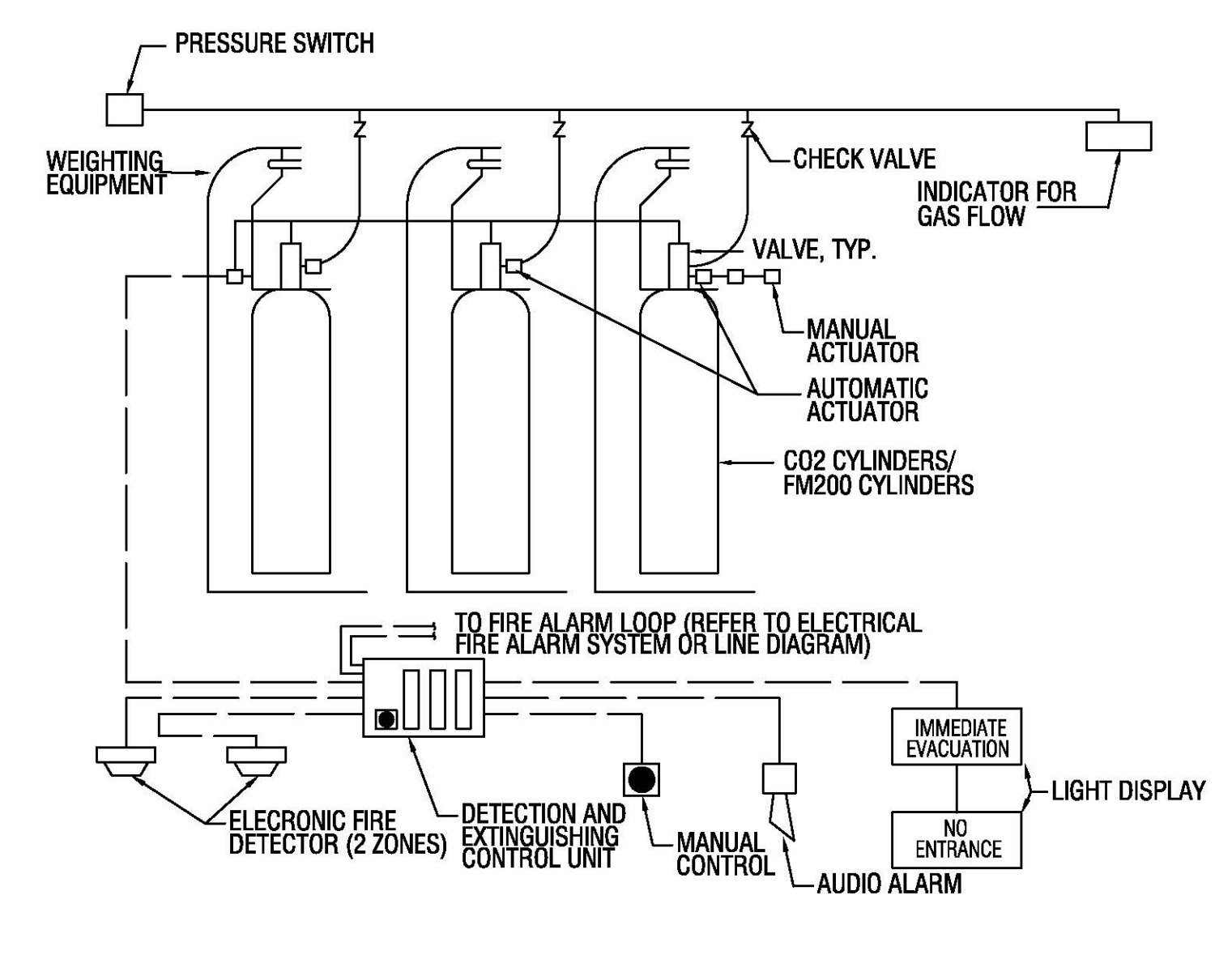
12 FM-200 & CO2 FLOODED SYSTEM SCHEMATIC G-PP002 N.T.S.
