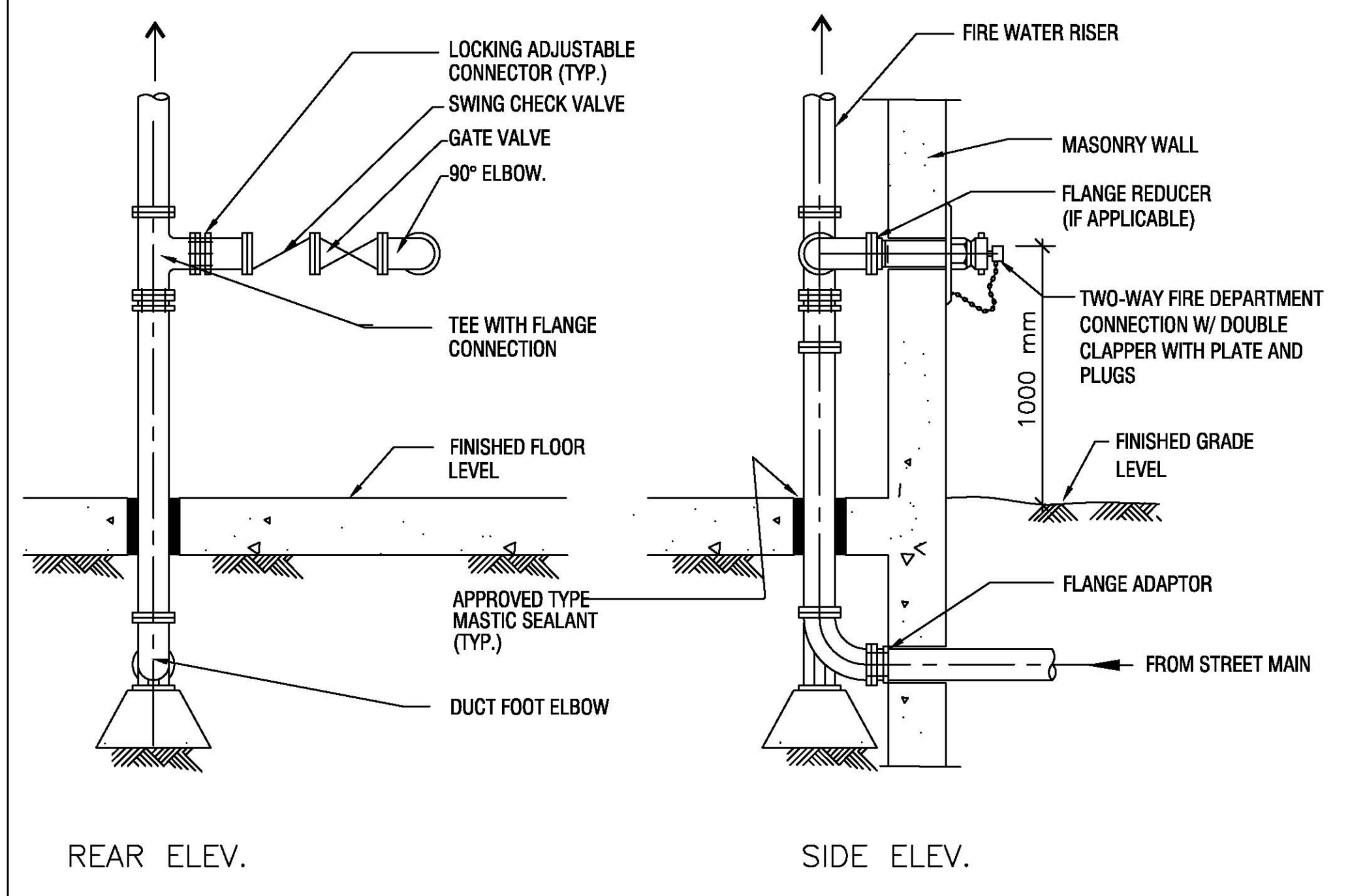
2 FIRE DEPARTMENT CONNECTION DETAIL G-PP002 N.T.S.
