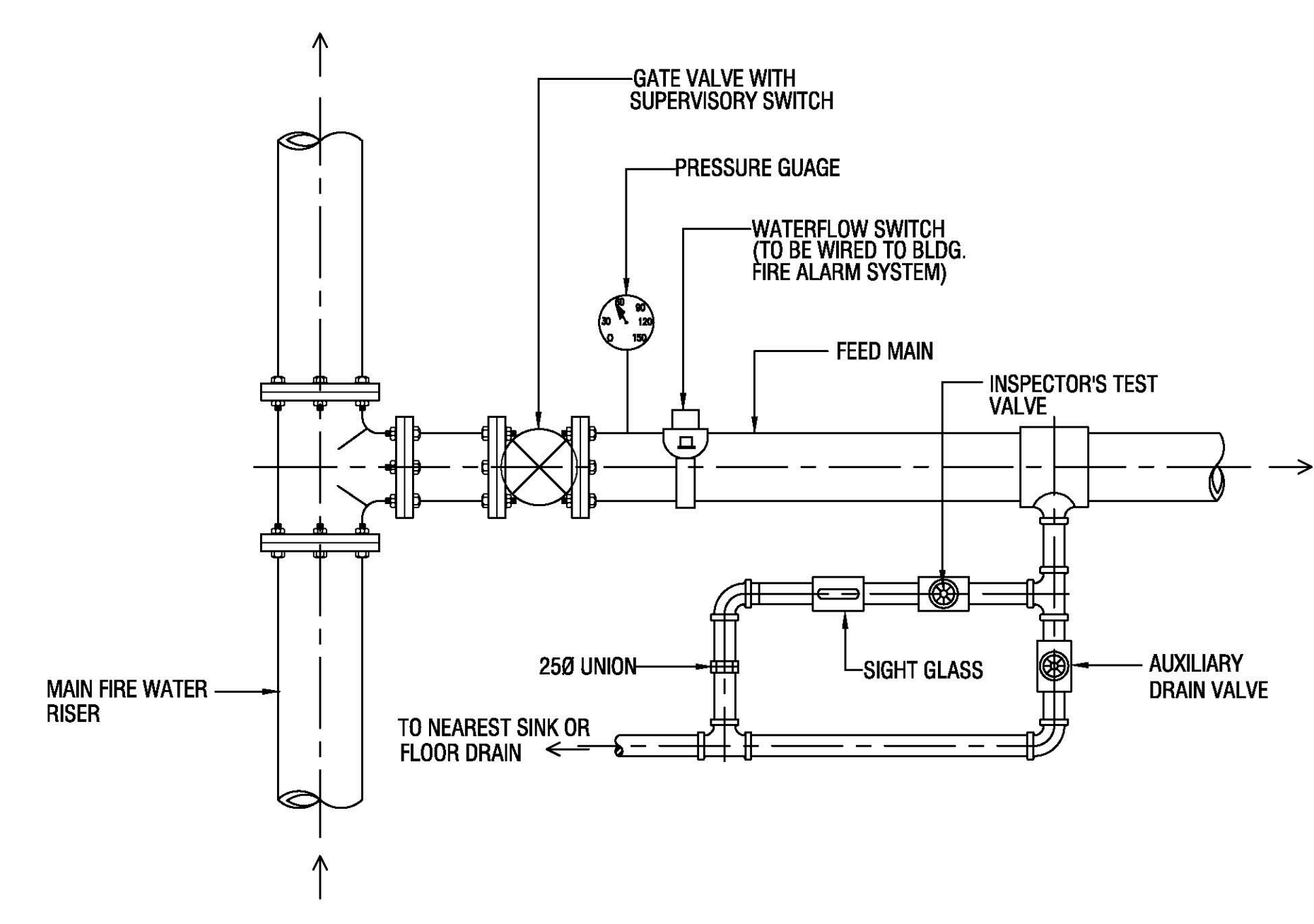
3 FLOOR CONTROL VALVE ASSEMBLY G-PP002 N.T.S.
