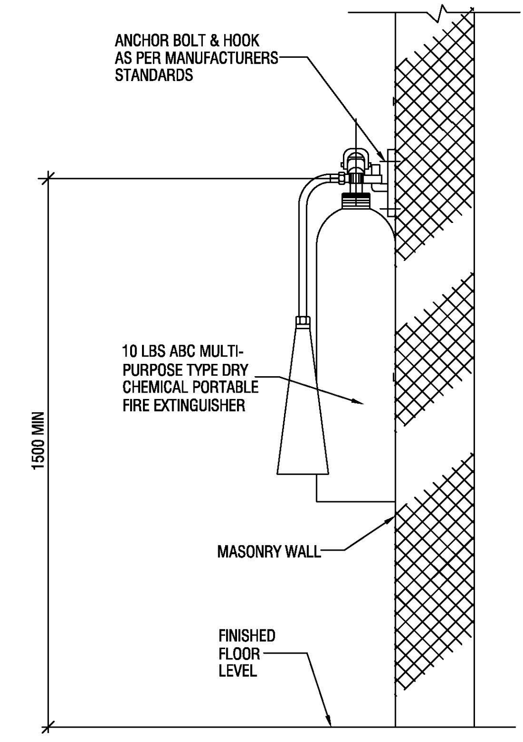
7 PORTABLE FIRE EXTINGUISHER MOUNTING DETAIL G-PP002 N.T.S.
