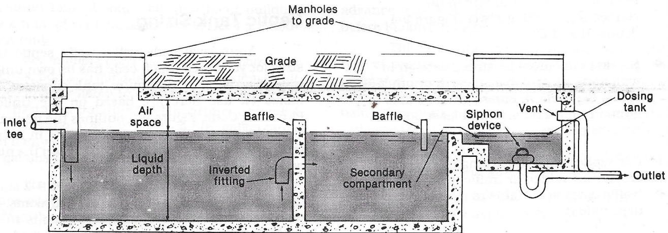
Detail C: Cross section of large septic tank with secondary compartment and dosing tank.
