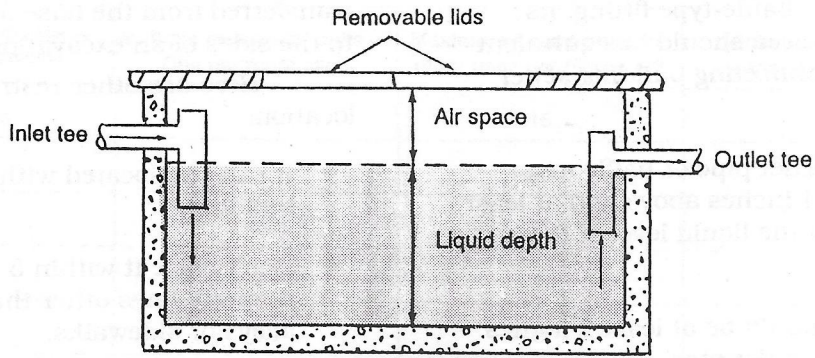
Detail A: Cross section of small septic tank
