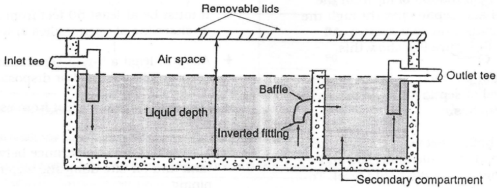
Detail B: Cross section of typical septic tank with secondary compartment
