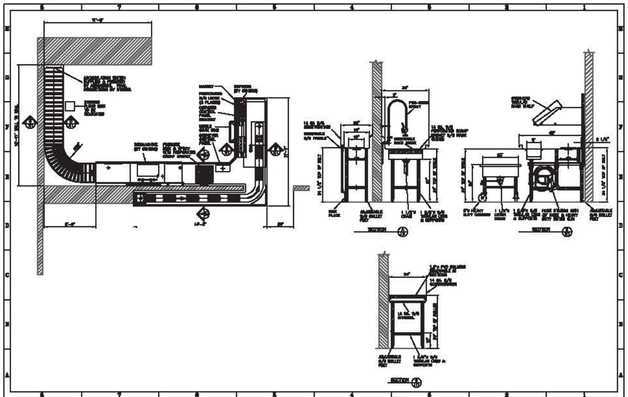
Soiled Tray Handling System: Tray return slat belt conveyor with soiled table and clean roller table
