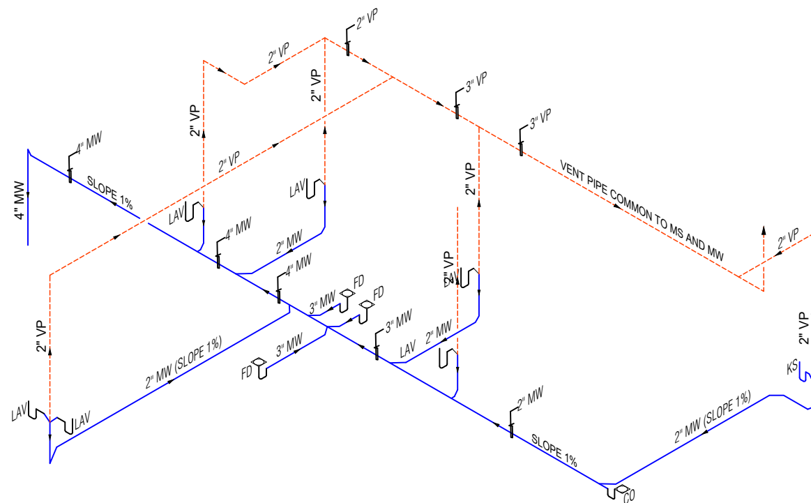
BATHROOM 3, 4, 5 & 6 WASTE PIPE ISOMETRIC
