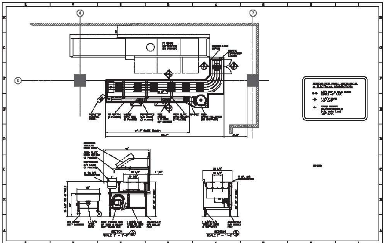
Soiled Tray Handling System: Dual slat belt scraping system. Also called parallel flow system or bussing conveyor
