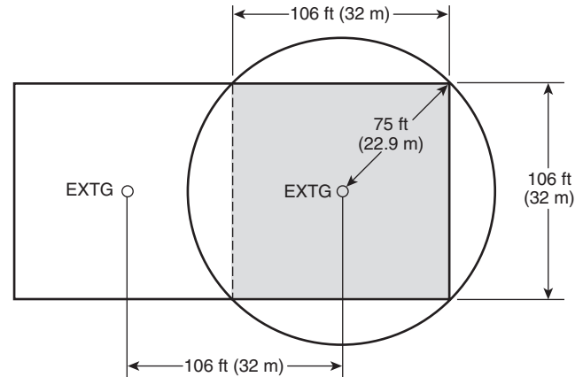
FIGURE E.3.4 Extinguishers Placed 106 ft (32 m) Apart to Comply with 75 ft (22.9 m) Travel Distance and 11,250 ft 2 (1045 m 2 ) Maximum Floor Area per Extinguisher.
