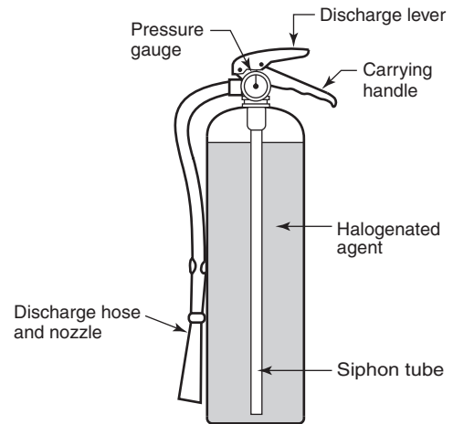
FIGURE D.4.4.1 Halogenated Agent-Type Stored-Pressure Fire Extinguisher.
