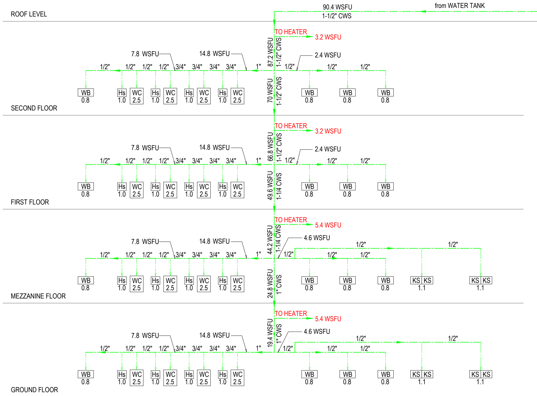
TOILET - 1 (GRID 1-2 & B-C)
